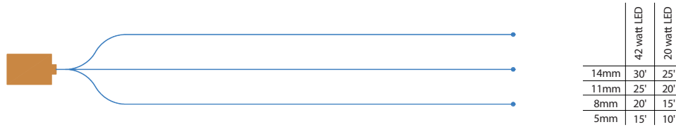
FIGURE 2. Fiber Lengths in Single-Ended Configuration
