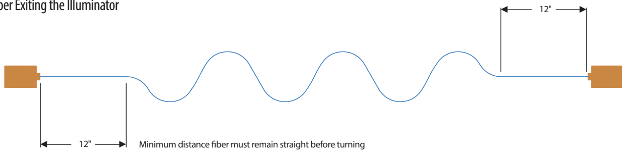
FIGURE 4. Fiber Exiting the Illuminator
