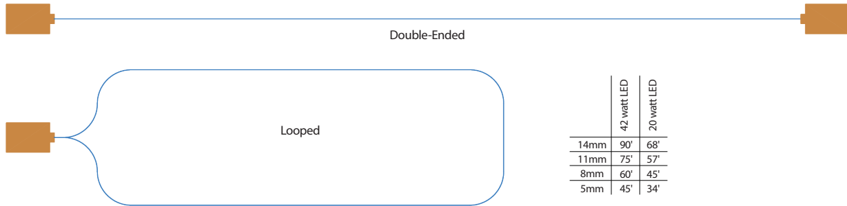
FIGURE 1. Fiber Lengths in Double-Ended / Looped Configuration
