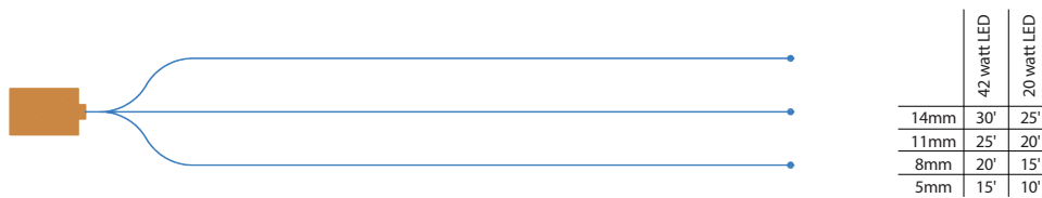
FIGURE 2. Fiber Lengths in Single-Ended Configuration
