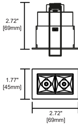
Trimmed Dual Cell
