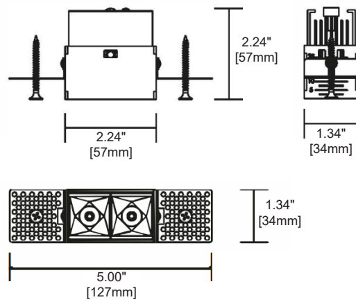
Trimless Sheetrock Dual Cell
