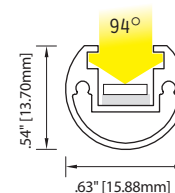
(Beam Angle based on 2RL fixture with Clear Acrylic lens)
